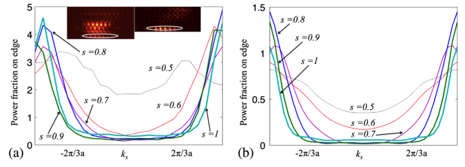
FIG. 5 (color online). Similar to Fig. 4, but for the zigzag edge.
